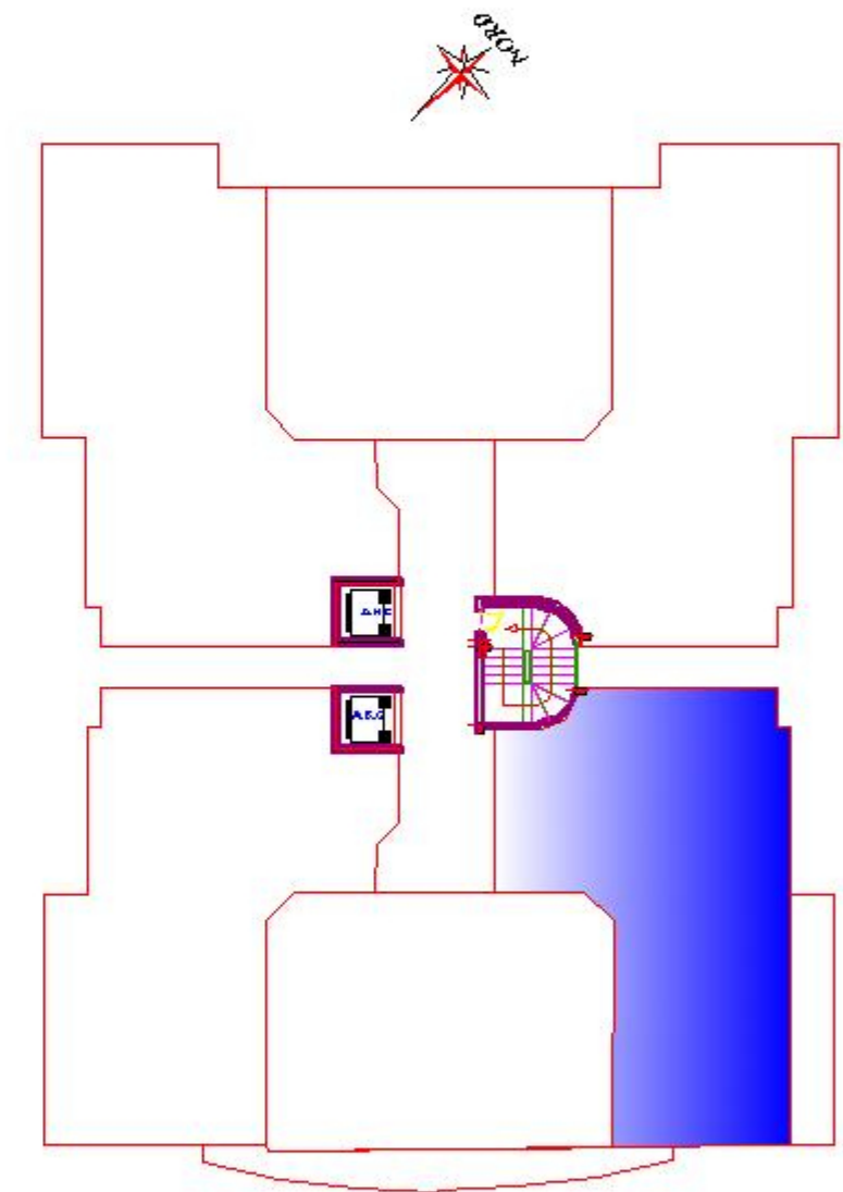
PLAN R+6
